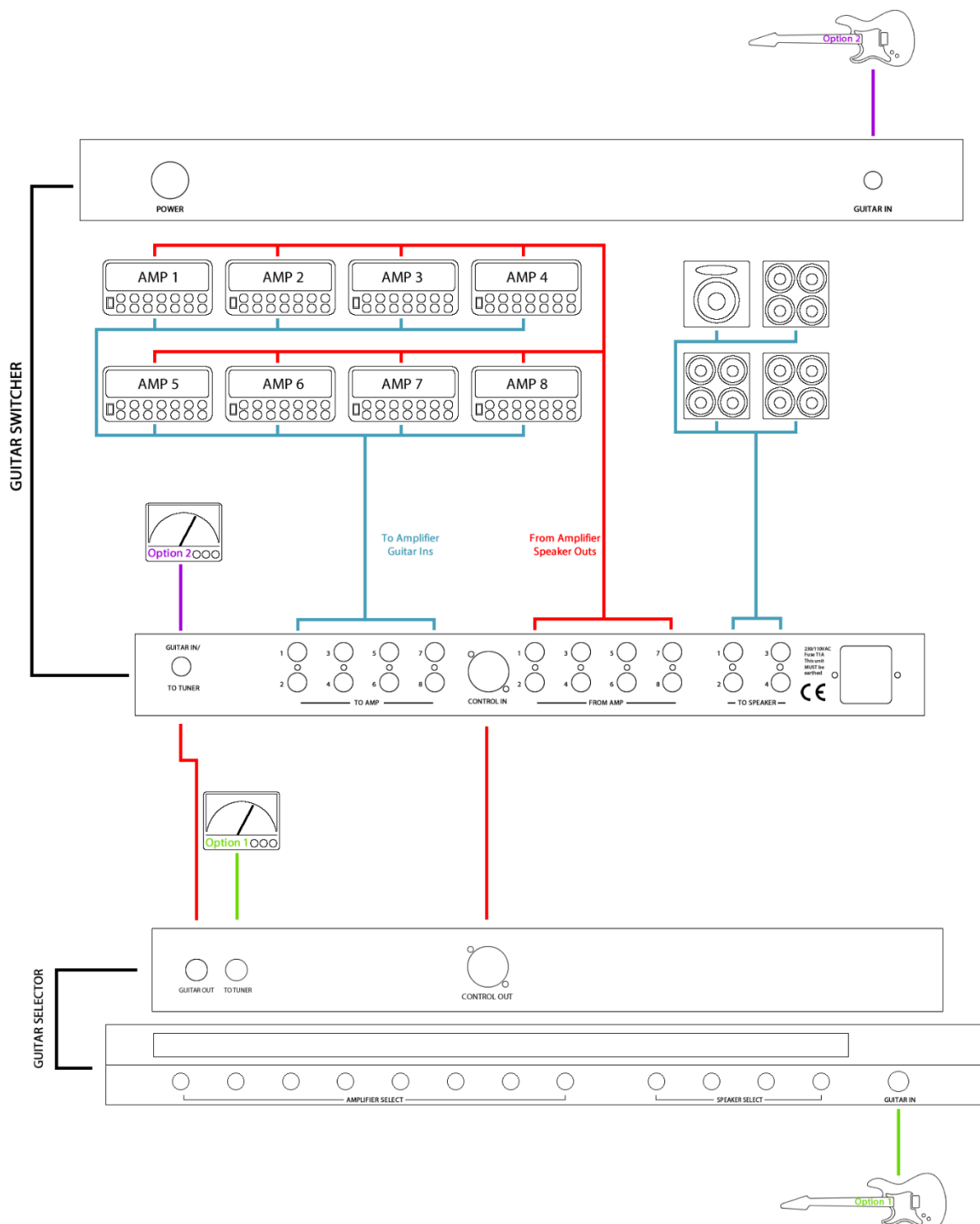
DACS HeadLine guitar switching system connection diagram
